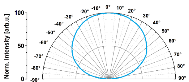
Radiation Pattern
