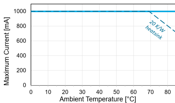
Maximum Ratings (1)
