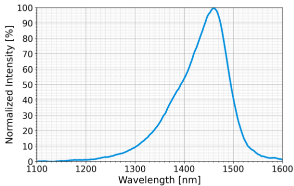
Optical Spectrum (at 100 mA)
