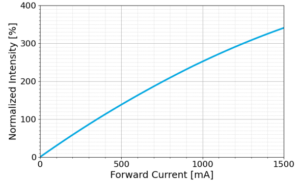
Relative Intensity vs. Forward Current
