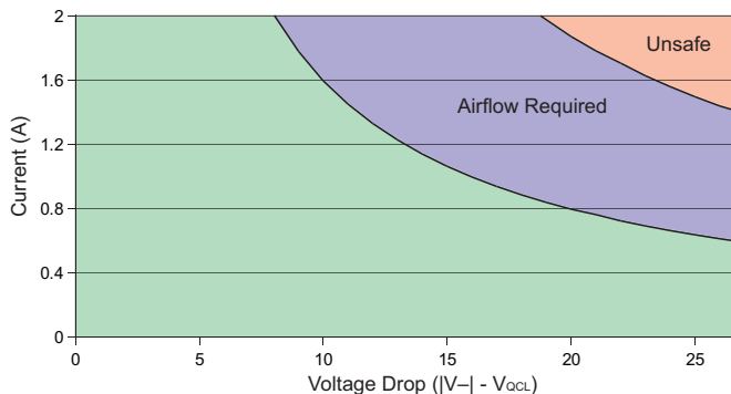
Figure 19. QCL2000 SOA Chart, at 25°C
