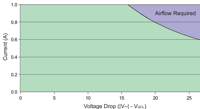
Figure 17. QCL1000 SOA Chart, at 25°C
