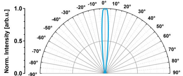
Radiation Pattern
