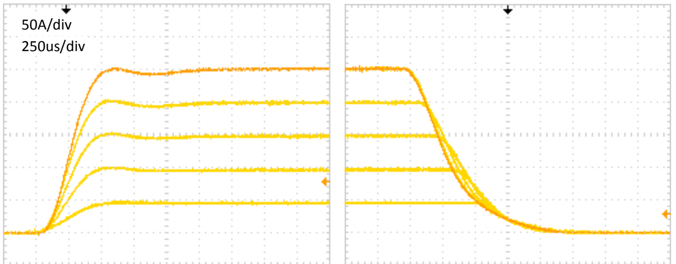
Figure 6 – Typical start up and stop sequence at V_{out} = 0.9-1.3V
