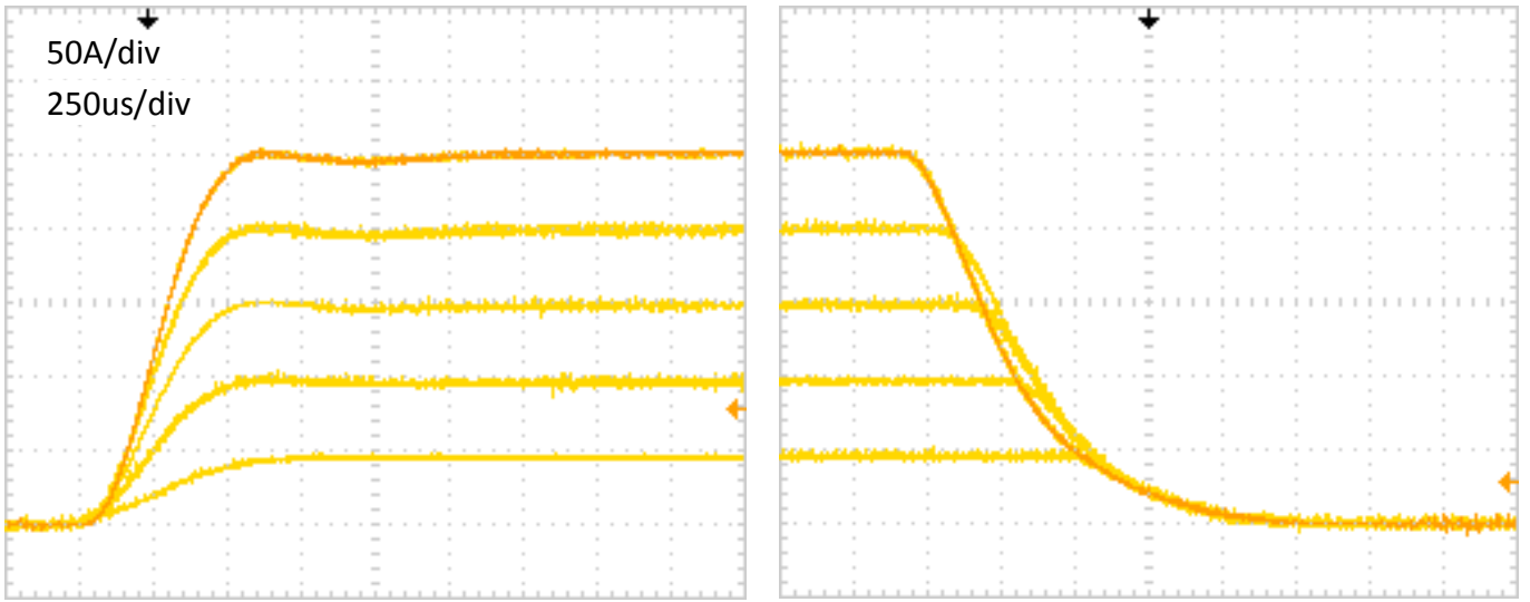
Figure 7 – Typical start up and stop sequence at V_{out} = 1.8-2.3V
