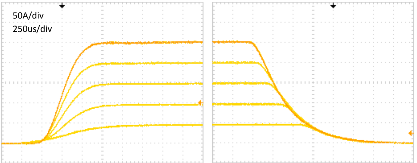
Figure 8 – Typical start up and stop sequence at V_{out} = 4.3-5.4V
