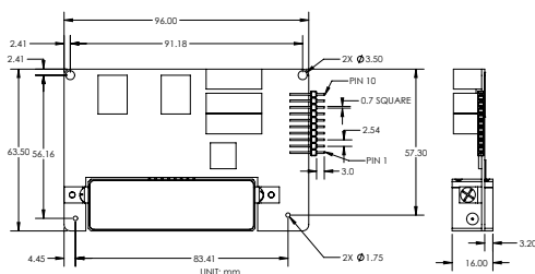
board
