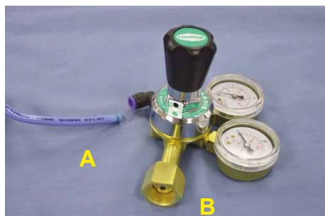
Propellant gas line connection.
