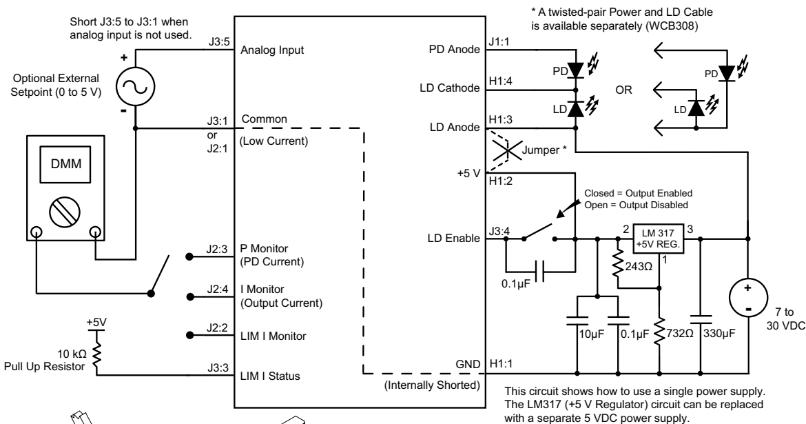
Figure 6. High-Compliance Laser Diode Operation PLD5K-CH and PLD10K-CH
