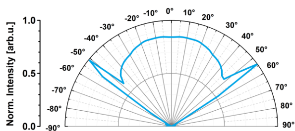
Radiation Pattern
