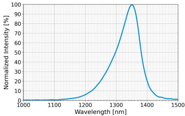
Optical Spectrum (at 100 mA)
