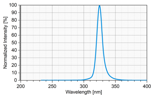
Optical Spectrum
