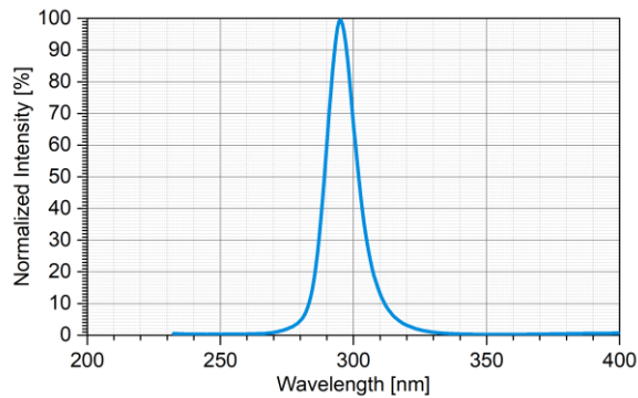
Optical Spectrum
