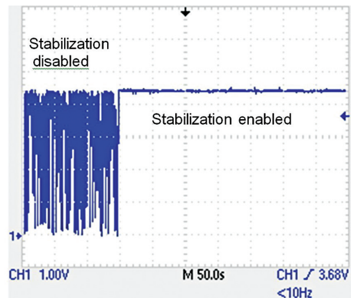
Figure 4. POS-002-I tracking of half-wave plate rotation at 45π rad/s.
