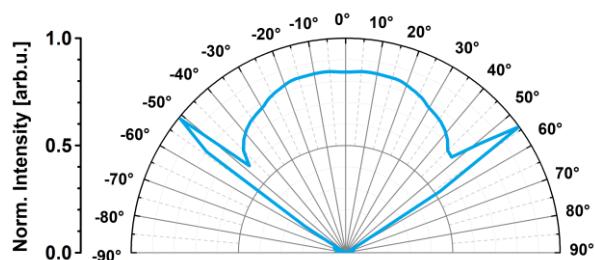
Radiation Pattern
