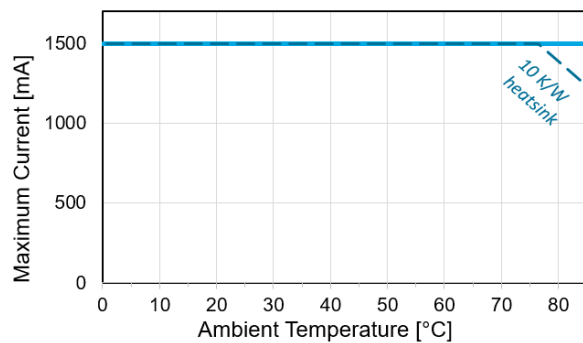
Maximum Ratings (1)
