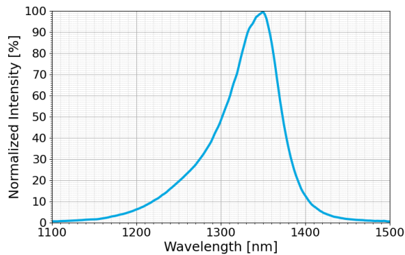
Optical Spectrum
