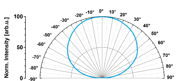
Radiation Pattern
