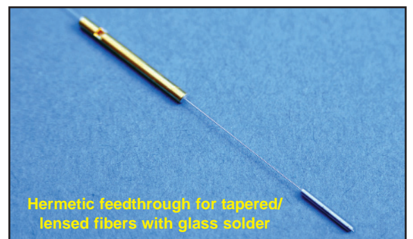
Single Channel Hermetically sealable patchcords with glass solder
