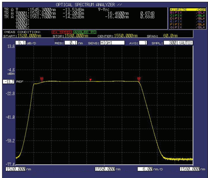
Figure 1. Output spectrum
