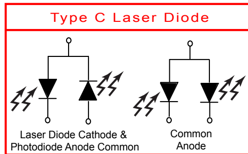
Figure 3. External connections for LDD 2P. Supports Type C laser diodes.
