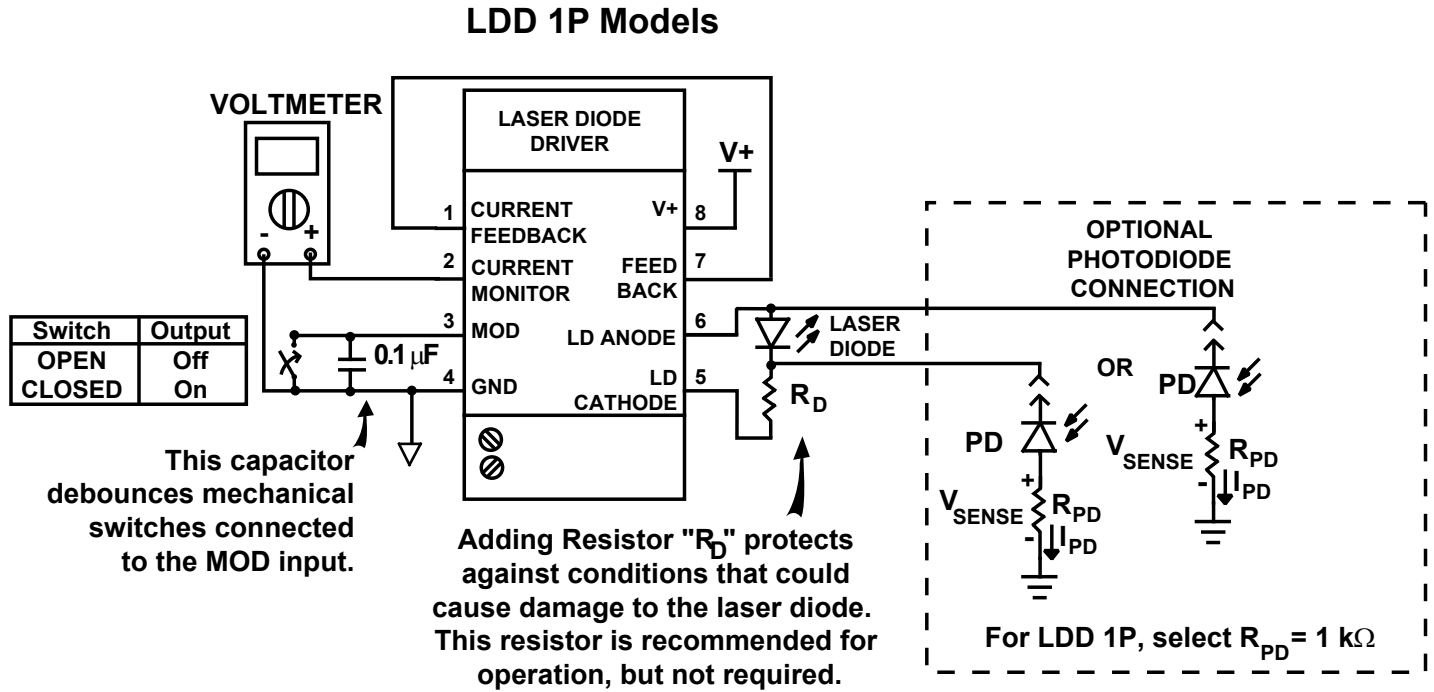
Figure 6. Wiring diagram for LDD 1P models. For use with Type A and Type B diode lasers.
