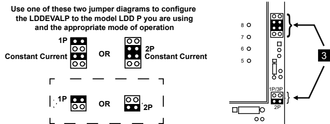
Figure 20. Properly configure the jumpers for the LDD P model being used.
