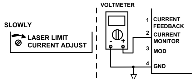
Figure 11. Set the Limit Current Adjust trimpot to the limit voltage.
