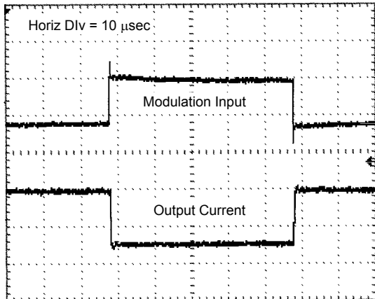
Figure 37. 10 kHz square wave response
