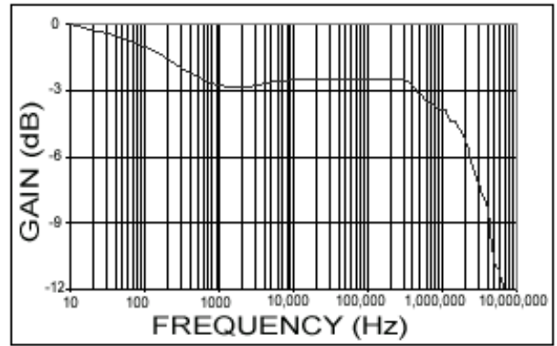
Figure 46. Large signal frequency response (Gain normalized to output at 10 Hz)
