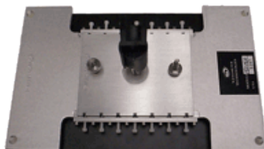
MT-RJ - 14 position
