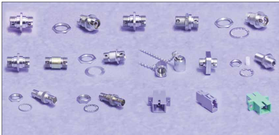
Sleeve-thru adapters for ultra, super, or angled connectors
