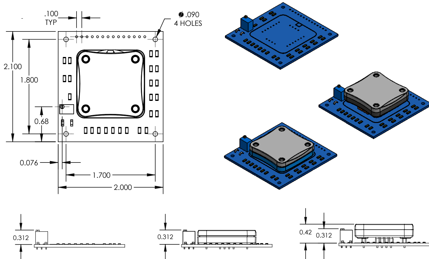
Figure 27. WTCPOEM Dimensions
