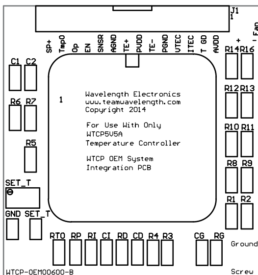
Figure 26. WTCPOEM Component Locator
