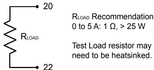
Figure 3. Test Load
