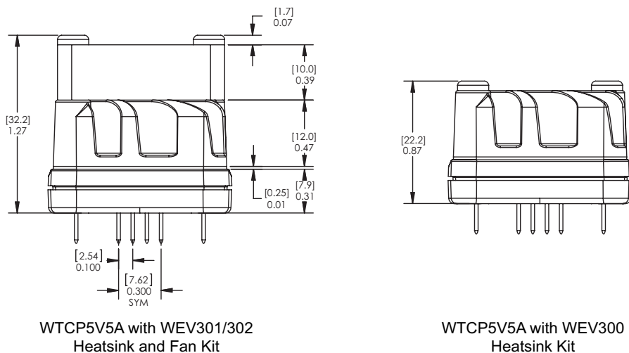
Figure 30. WTCP5V5A with WEV301/302 and WEV300 Thermal Solution Kits
