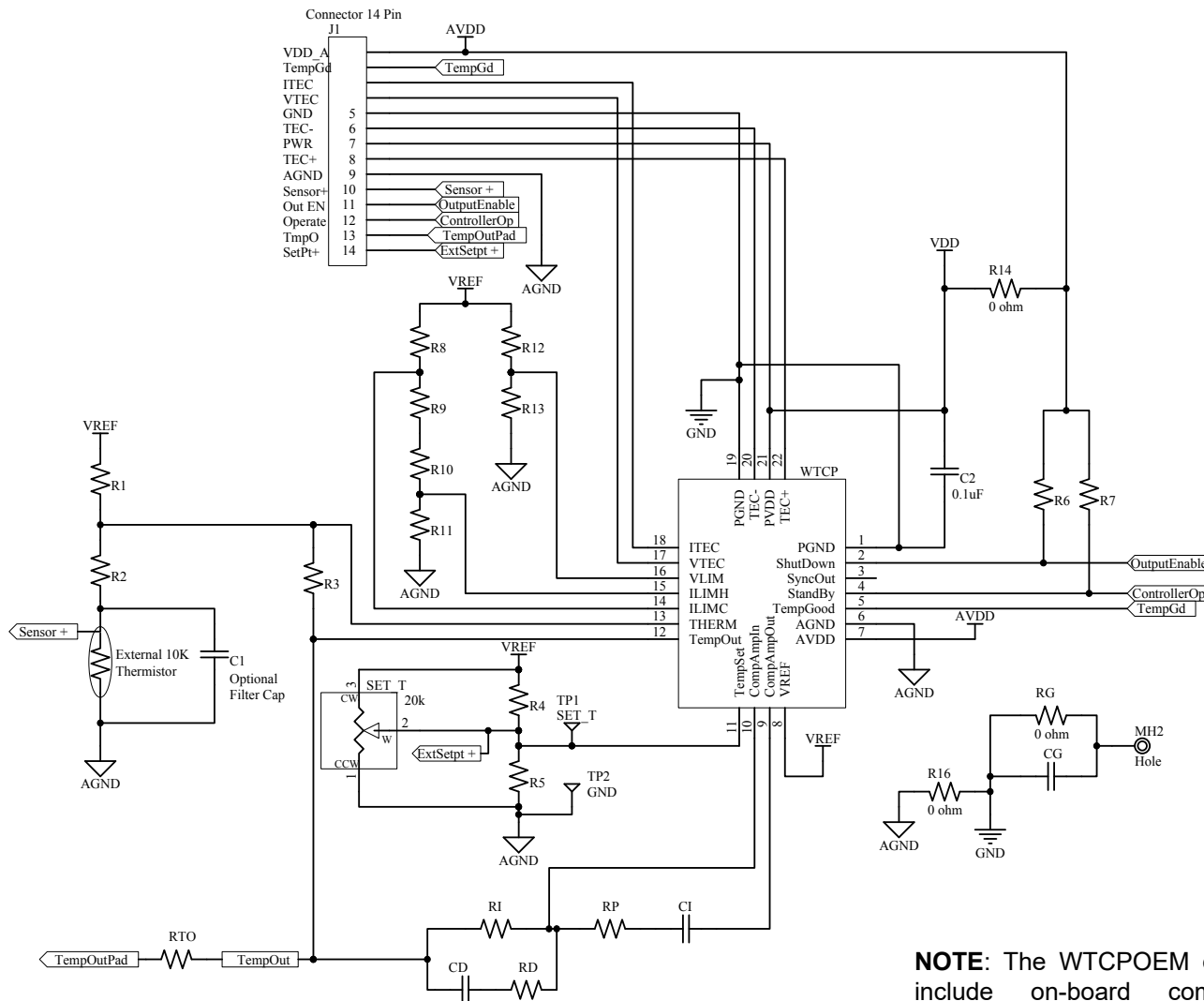
Figure 25. WTCPOEM Schematic
