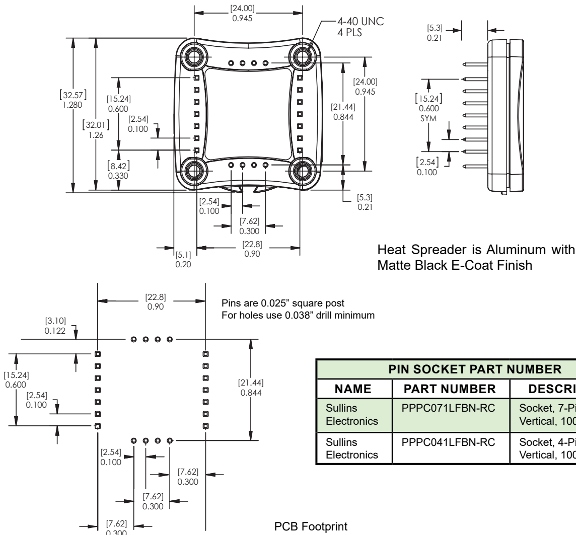
Figure 29. WTCP5V5A Dimensions
