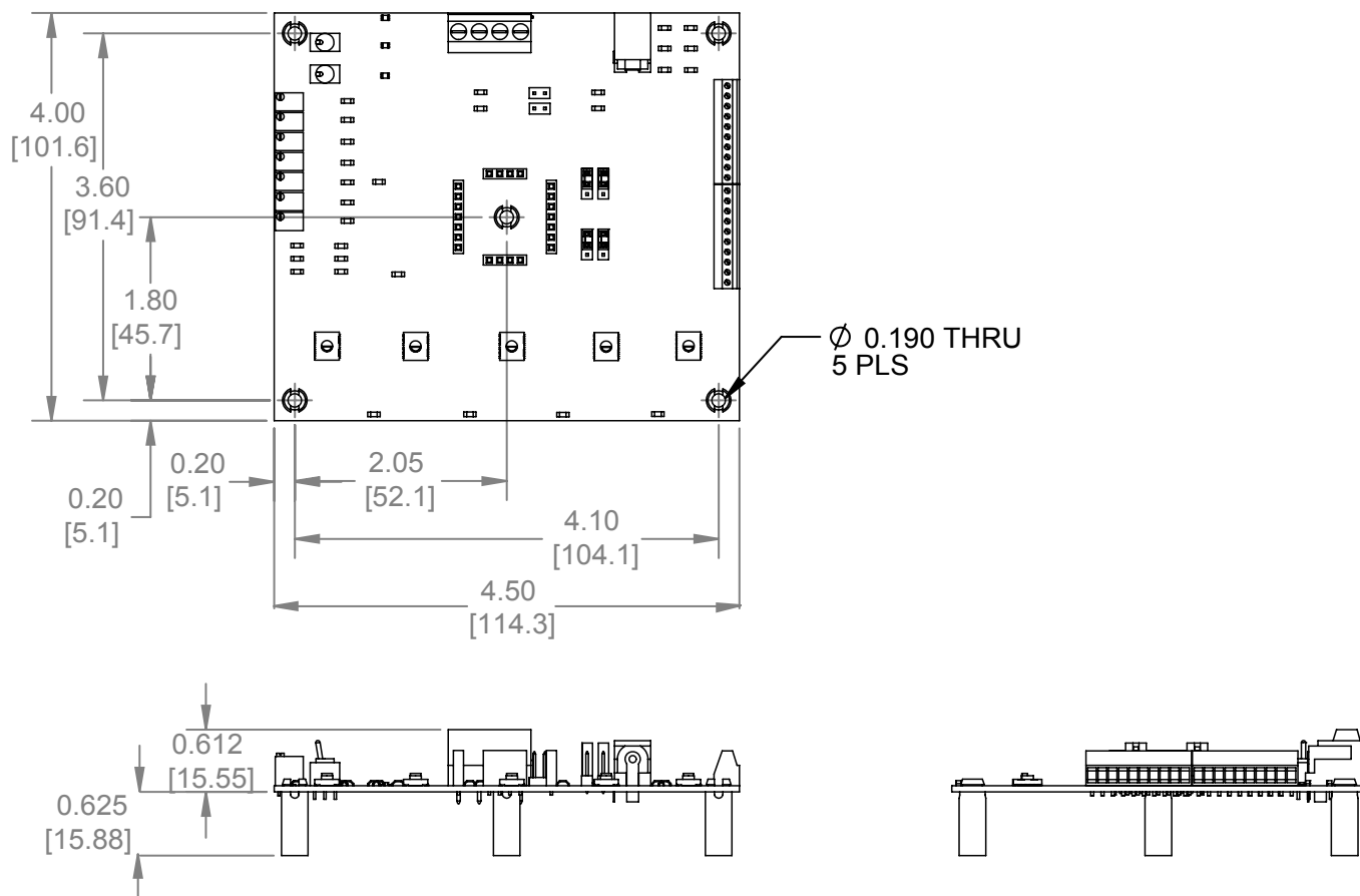
Figure 28. WTCP5V5A with WEV301/302 and WEV300 Thermal Solution Kits
