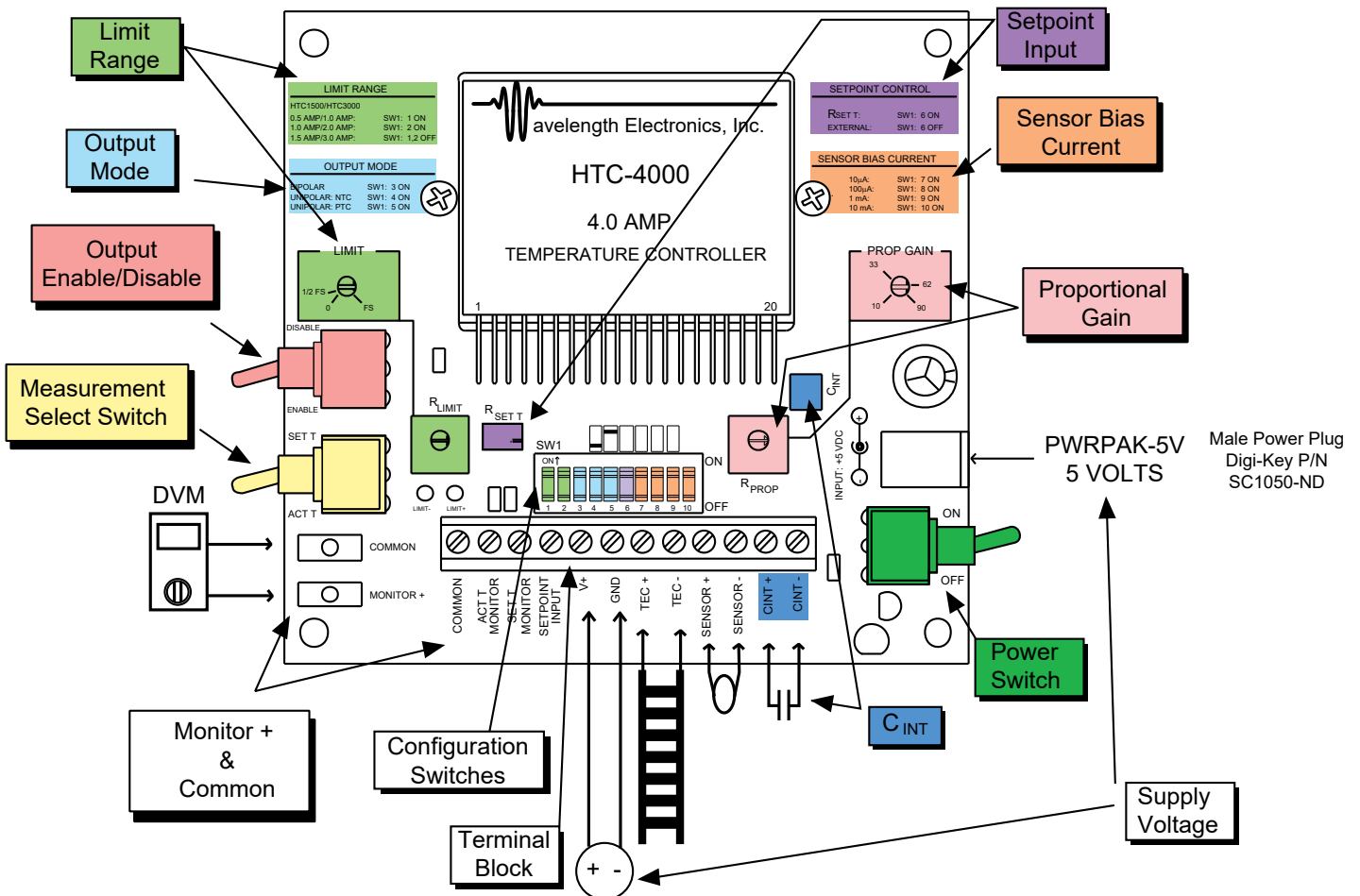
Figure 6. HTCEVALPCB Board Top View
