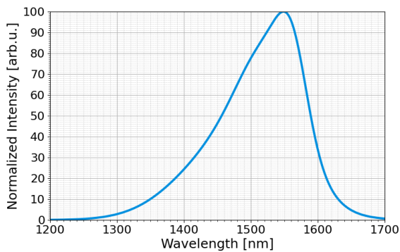
Optical Spectrum (at 100 mA)
