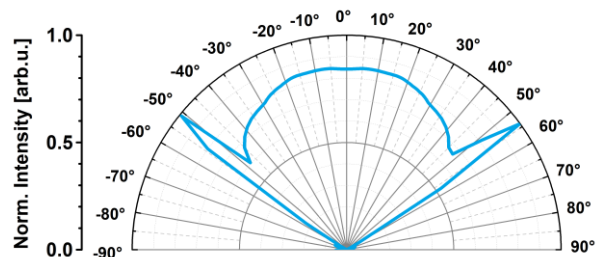
Radiation Pattern
