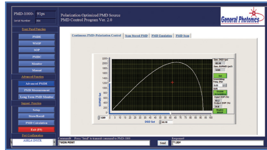
Figure 2. Quasi-continuous PMD control
