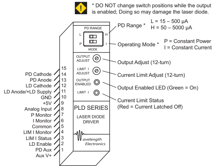
Figure 1. PLD Driver Controls
