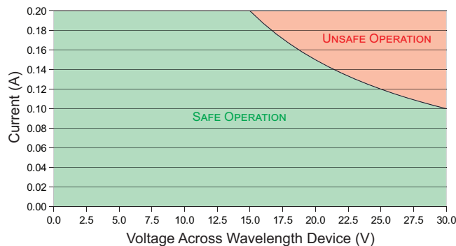
Figure 23. SOA for PLD200
