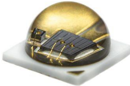
High Power LED with Silicone Glob Top
