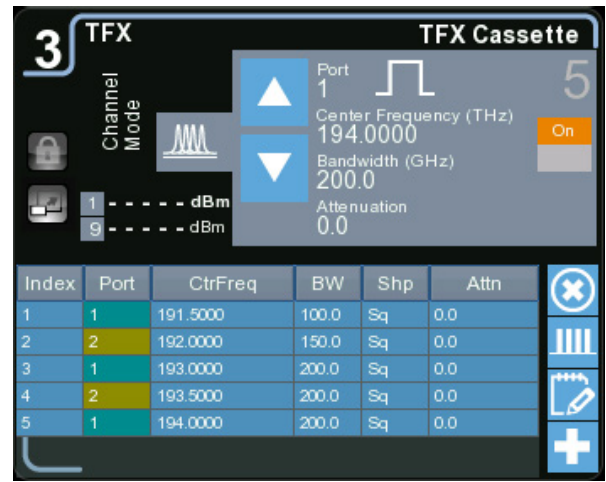
Figure 3. The MAP-220 GUI
